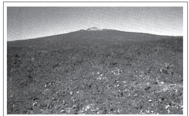
Cinder Cone
