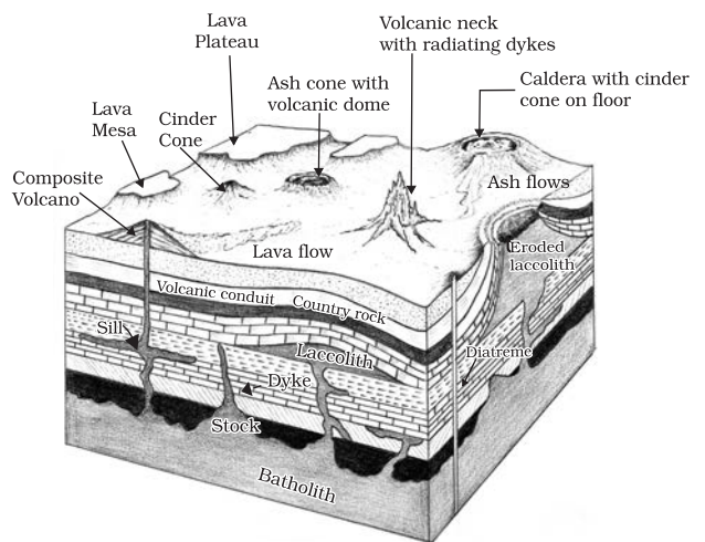
Figure 3.4 : Volcanic Landforms
