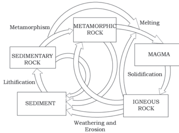
Fig 5.1 : Rock Cycle
