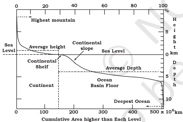
Figure 4.1 : Ocean Floor
