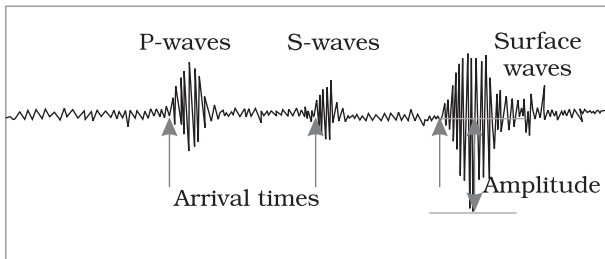
Figure 3.1 : Earthquake Waves
