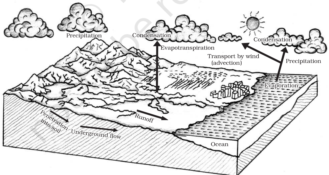
Figure 13.1 : Hydrological Cycle
