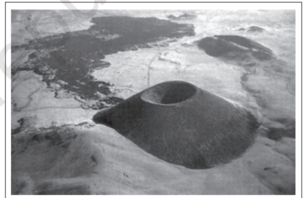
Shield Volcano
