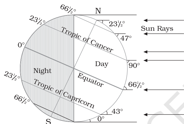
Figure 9.1 : Summer Solstice
